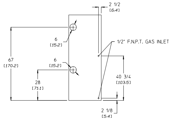
REAR VIEW (GAS AND ELECTRIC)
