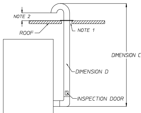
VERTICAL DUCTING
