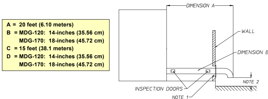
HORIZONTAL DUCTING
